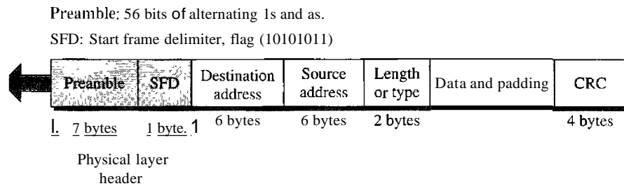
Figure 13.4 802.3 MAC frame
